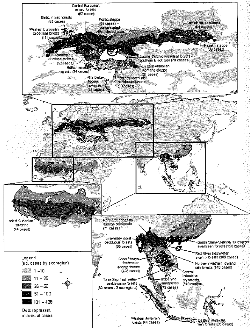
Figure 24.4. Map showing the 25 ecoregions with large numbers of avian influenza cases (November 2003–November 2006). (A) Eurasia; (B) Southeast Asia; (C) Africa. Dots represent individual cases (figure reprinted with permission © Centers for Disease Control and Prevention. Emerging Infectious Diseases , 13, 1269–1271).
