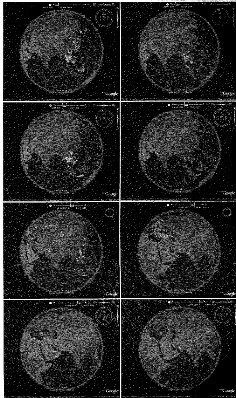
Figure 24.3. Snapshots of Declan Butler's maps of bird flu occurrences between 2003–2006.
