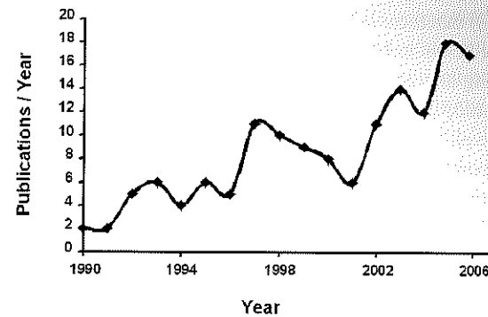
Figure 24.1. The number of publications per year revealed by a search using the Web of Science, with the search terms "parasite" and "primate."
