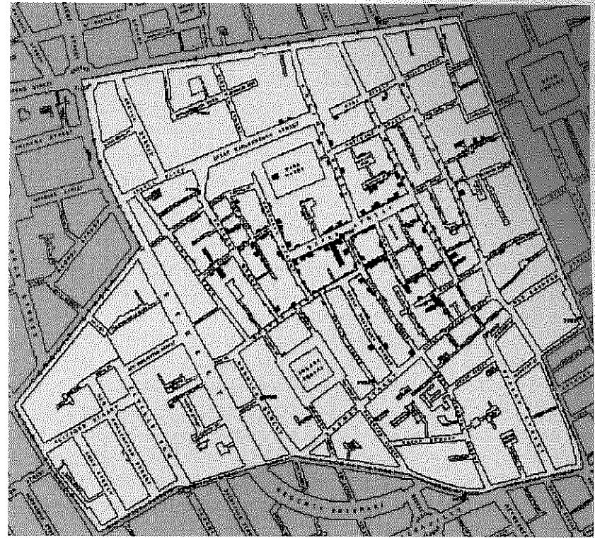
Figure 24.2. Modified map from John Snow's (1855) map of cholera incidences (each case is shown as a bar) and location of hand pumps.
